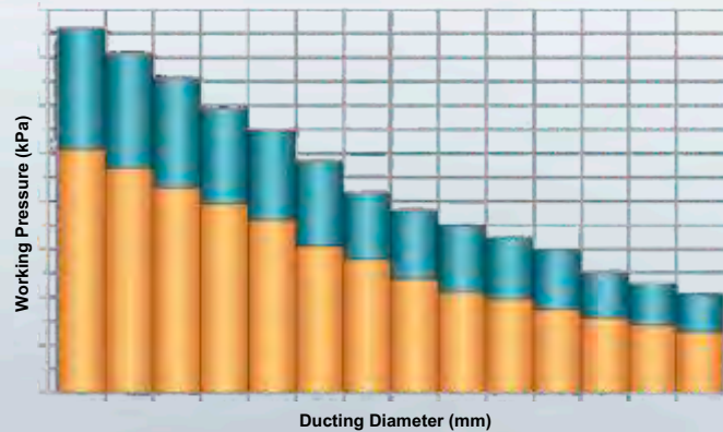
Ventilation Ducting Pressure Chart Highest permitted working pressure
